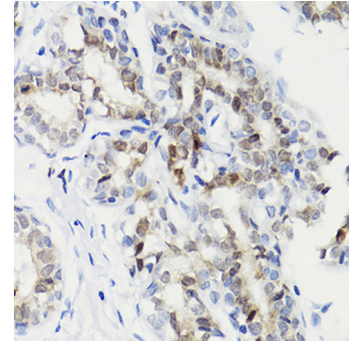
Fig. 4. Immunohistochemistry of paraffin-embedded human breast cancer using Phospho-Stat3-S727 antibody at dilution of 1:100 (40x lens).
