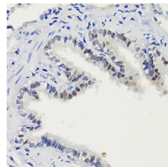
Fig. 2. Immunohistochemistry of paraffin-embedded rat lung using Phospho-Stat3-S727 antibody at dilution of 1:100 (40x lens).
