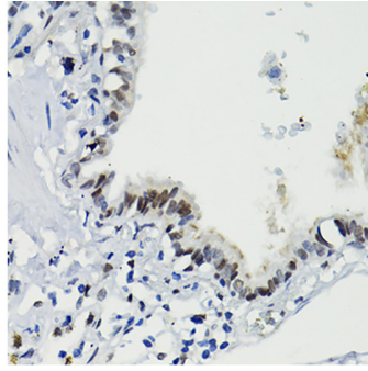
Fig. 3. Immunohistochemistry of paraffin-embedded human lung using Phospho-Stat3-S727 antibody at dilution of 1:100 (40x lens).
