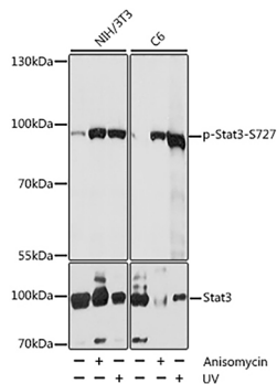
Fig. 1. Western blot analysis of extracts of various cell lines, using Phospho-Stat3-S727 antibody at 1:1000 dilution or STAT3 antibody at 37 °C room temperature for 15-30 minutes. C6 cells were treated by Anisomycin at 37 °C room temperature for 15-30 minutes. Secondary antibody: HRP-labeled Goat Anti-Rabbit IgG(H+L) (A0208) at 1:1000 dilution. Lysates/proteins: 25µg per lane. Blocking buffer: QuickBlock™ Blocking Buffer (P0231). Detection: BeyoECL Star (P0018A). Exposure time: 1s.
